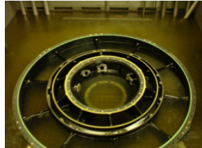
immersion degreasing
